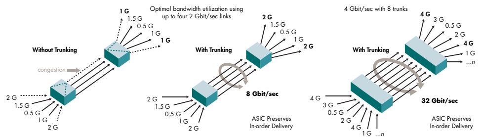
Figure 1. ISL Trunking with 1, 2, and 4 Gbit/sec links
